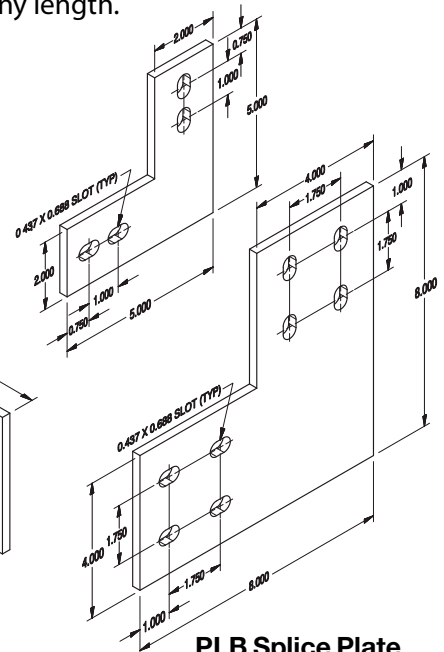
PLB Splice Plate
