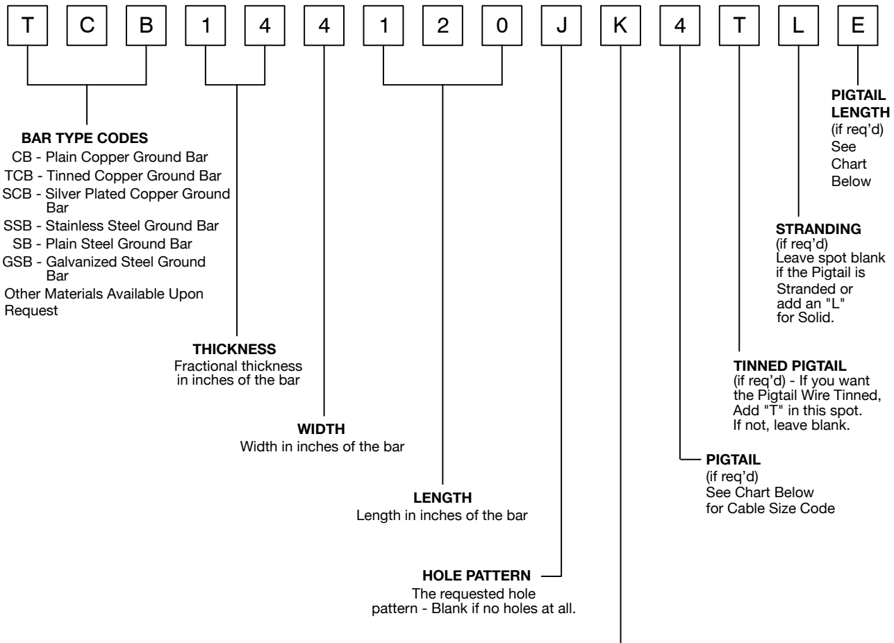
ASSEMBLY TYPE CODES
